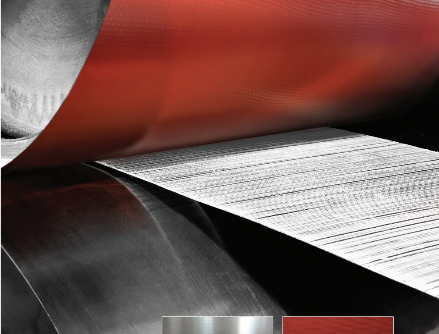
ThermoPress HB double belt press: the quality of a steel belt on a Teflon® press
